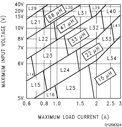
FIGURE4.LM2596/LM2596HV-3.3
