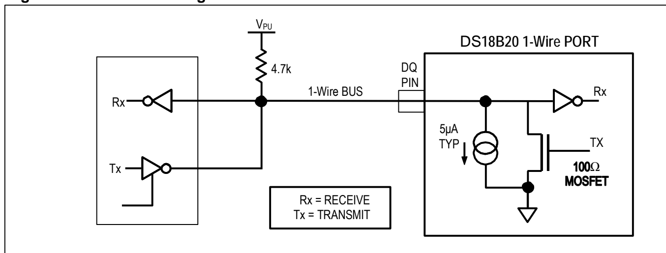
Figure 10. Hardware Configuration
