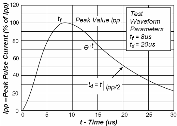
Fig3. Pulse Waveform
