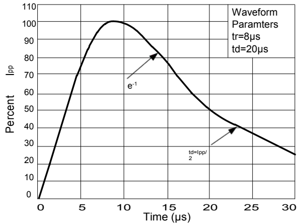
Figure 3: Pulse Waveform
