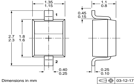
PESD5V0L1UA (SOD323)
