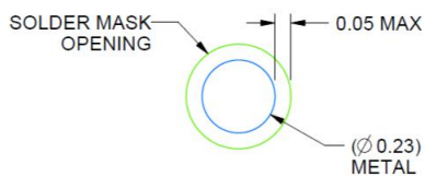
NON-SOLDER MASK DEFINED (PREFERRED)
