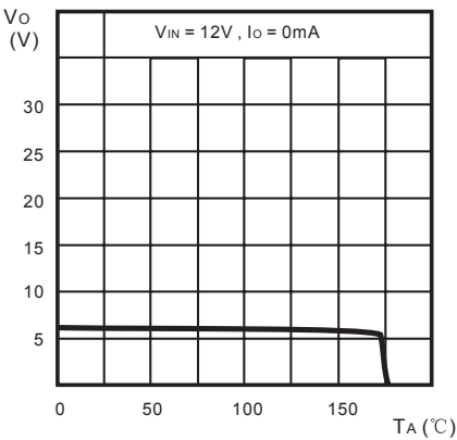
Thermal Shutdown
