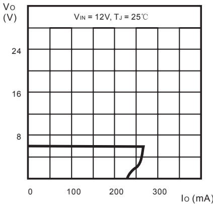
Load Characteristics
