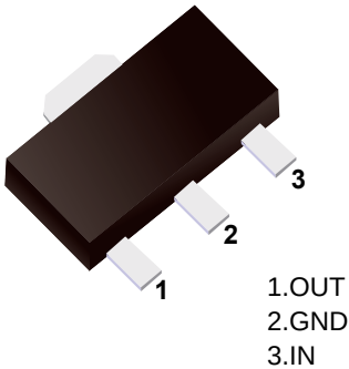
Simplified outline(SOT-89)
