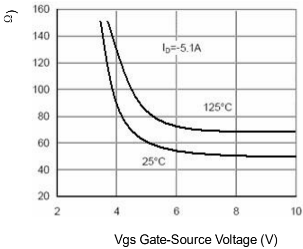
Figure 9 Rdsn vs Vgs
