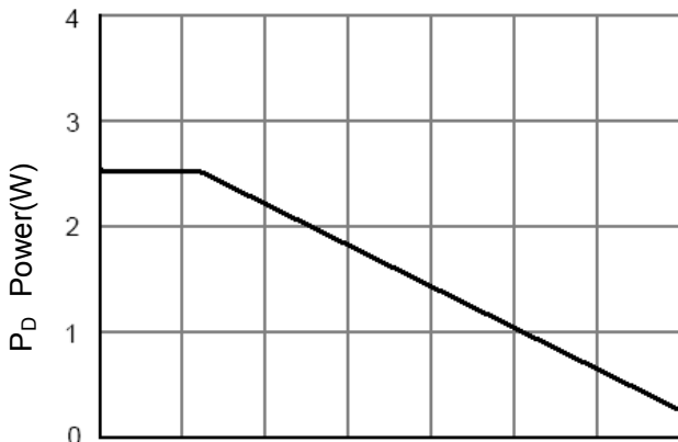
Figure 3 Power Dissipation
