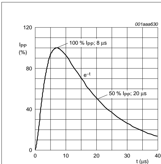
Fig 1. 8/20 μs pulse waveform according to IEC 61000-4-5
