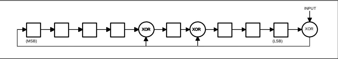
Figure 9. CRC Generator
