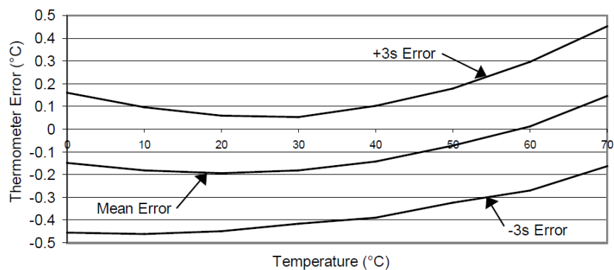
DS18B20 Typical Error Curve
