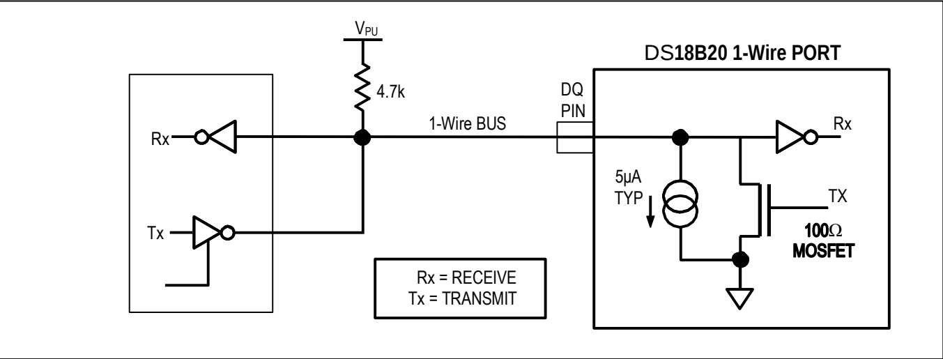
Figure 10. Hardware Configuration
