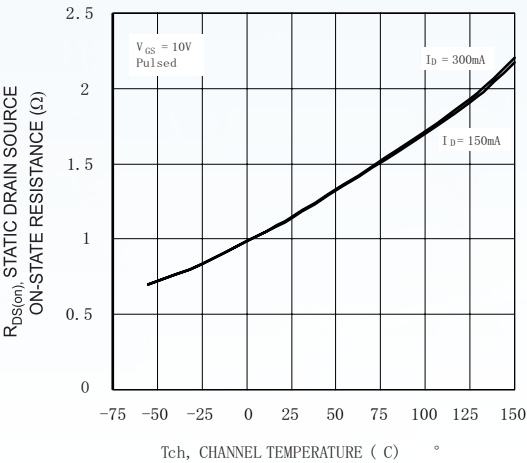
Fig. 7 Static Drain-Source On-State Resistance vs. Channel Temperature
