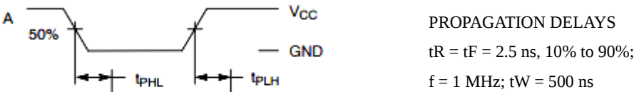
Figure 3. Switching Waveforms
