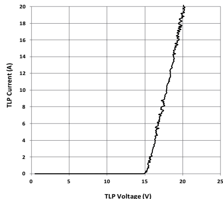
AQ12 Transmission Line Pulsing(TLP) Plot
